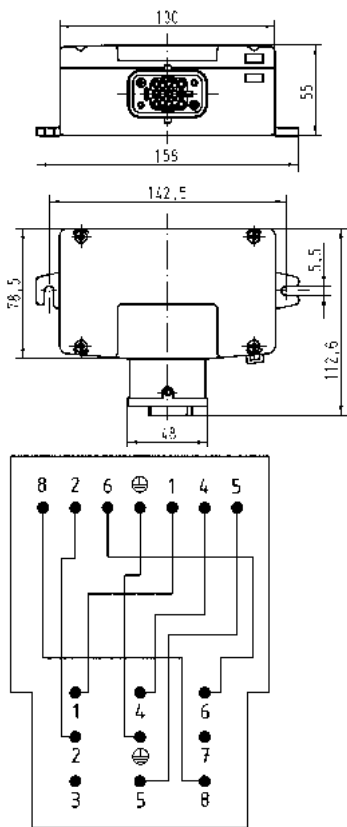
Wiring diagram
