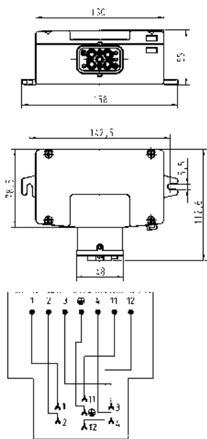
Wiring diagram
