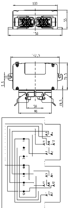
Wiring diagram
