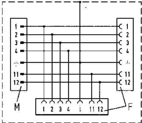
Wiring diagram
