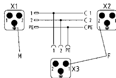
Wiring diagram
